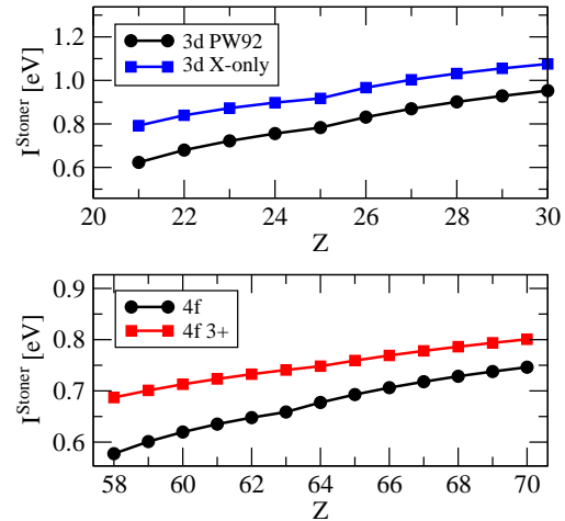
FIG. 4: Shell-Stoner integrals for the 3d and 4f atoms. For explanations see text.
